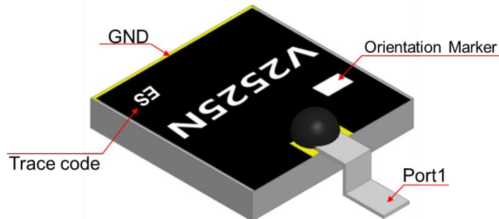
Figure 1. V2525N (Top View)
