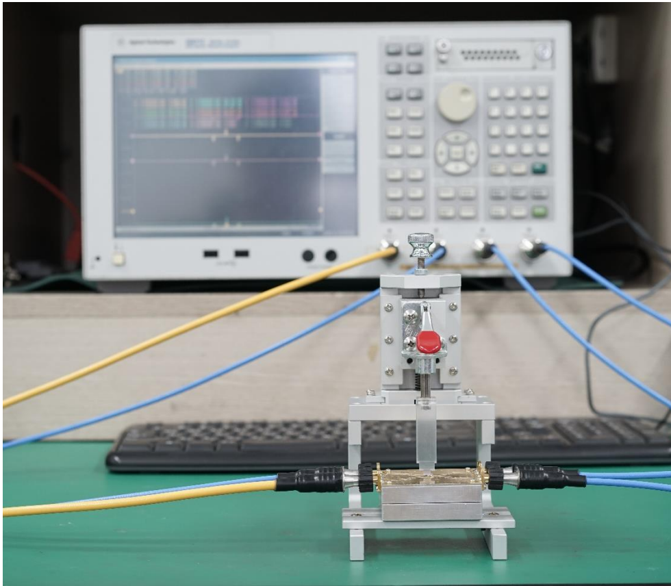
Figure 3. Test Setting to Measure the V2525N S-parameters
