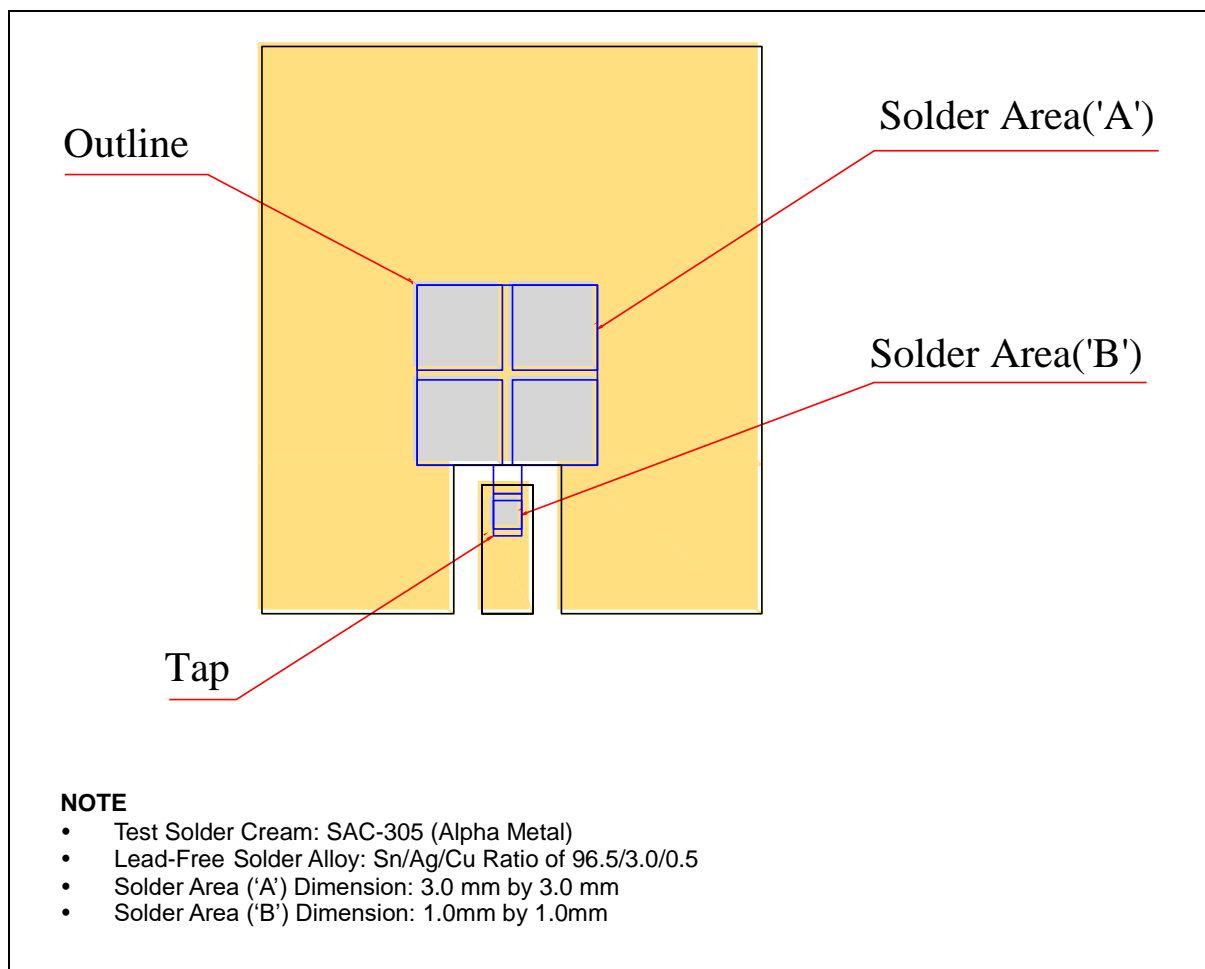
Figure 6. Recommended PCB Layout and Solder Mask Pattern
