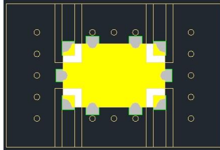
Figure 11. Placing the RCP450A03 on the 11 Points of the PCB Surface
