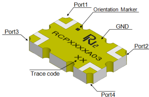
Figure 1. RCP450A03 (Top View)
