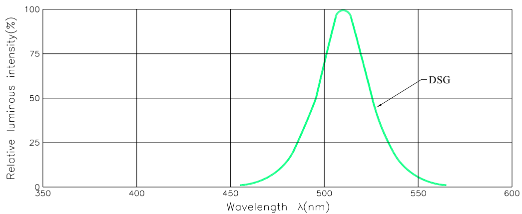
Spectrum Distribution
