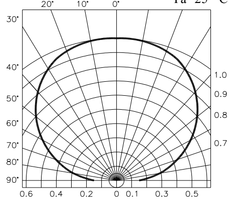
Radiation Diagram
