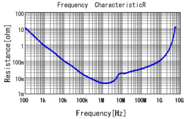
GRM21BR61H475ME51 R DCOV, 25degC
