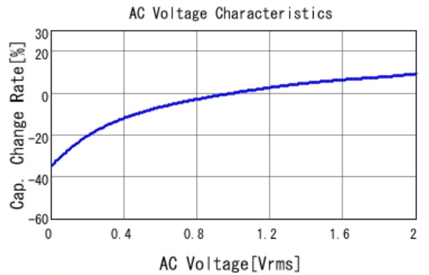
GRM21BR61H475ME51 C-AC Voltage capchange, DCOV, 25
