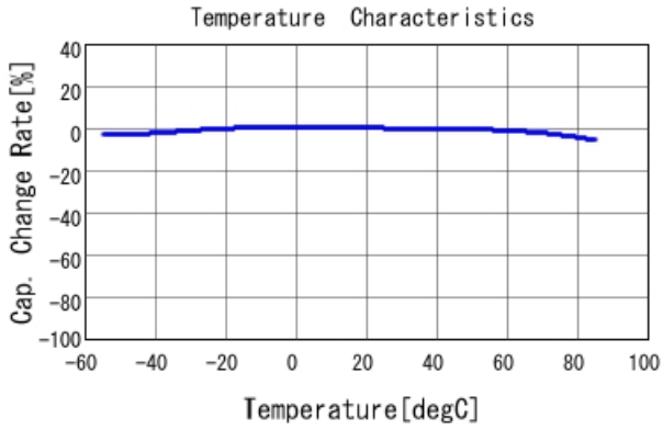
GRM21BR61H475ME51 C-Temp. capchange, DC0.0V, AC1.C
