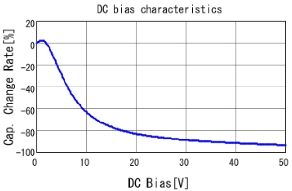
GRM21BR61H475ME51 C-DC bias capchange, 25.0degC, A
