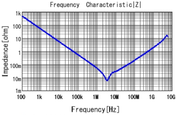
GRM21BR61H475ME51 |Z| DCOV, 25degC
