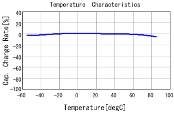
GRM21BR61H475KE51 C-Temp. capchange, DC0.0V, AC1.C
