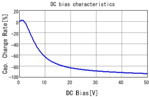
GRM21BR61H475KE51 C-DC bias capchange, 25.0degC, A
