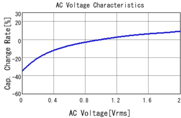
GRM21BR61H475KE51 C-AC Voltage capchange, DCOV, 25
