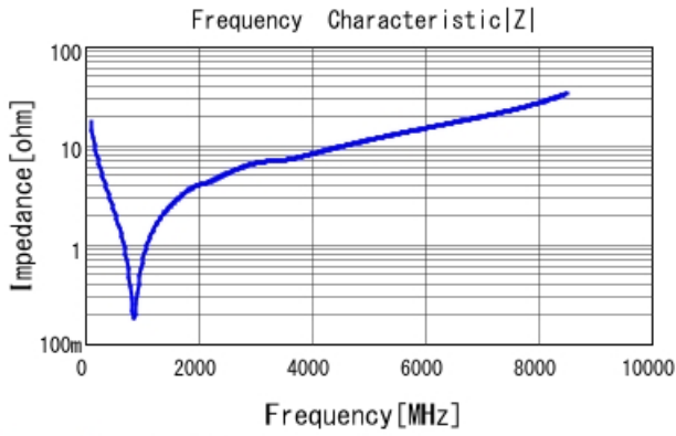
GRM1555C1H910JA01 |Z| DCOV, 25degC
