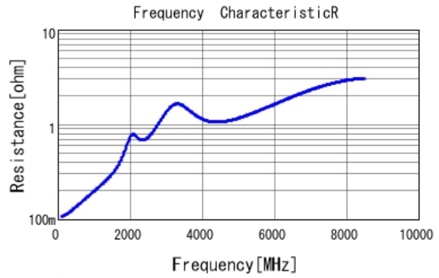
GRM1555C1H910JA01 R DCOV, 25degC
