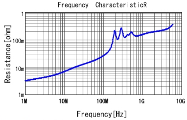
GRM1555C1H822GE01 R DCOV, 25degC
