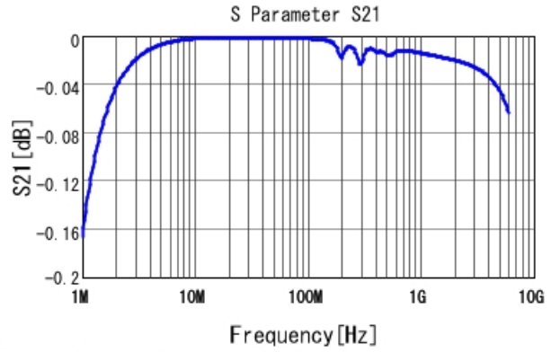
GRM1555C1H822GE01 S21 DCOV, 25degC
