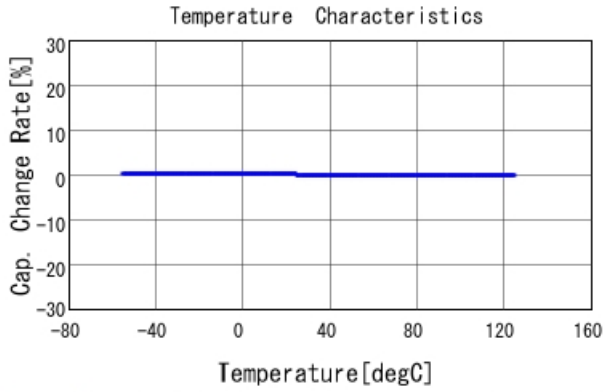
GRM1555C1H822GE01 C-Temp. capchange, DCOV, AC1Vrms
