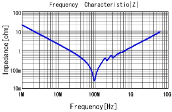
GRM1555C1H822GE01 |Z| DCOV, 25degC
