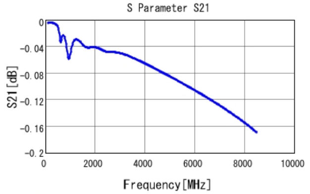
GRM1555C1H821GA01 S21 DCOV, 25degC
