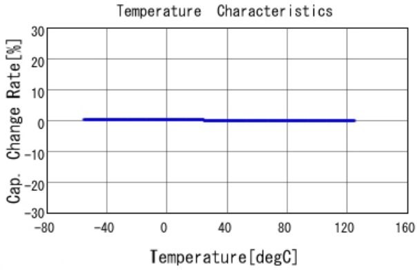
GRM1555C1H821GA01 C-Temp. capchange, DCOV, AC1Vrms
