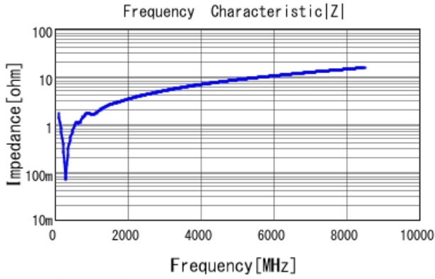
GRM1555C1H821GA01 |Z| DCOV, 25degC
