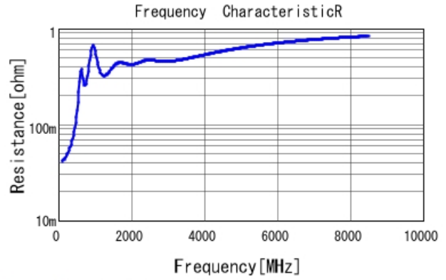
GRM1555C1H821GA01 R DCOV, 25degC
