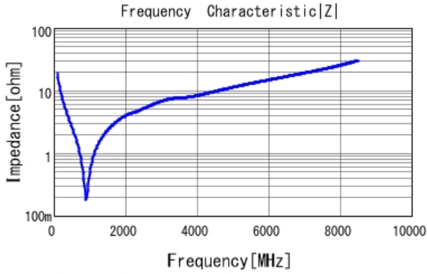
GRM1555C1H820JA01 |Z| DCOV, 25degC
