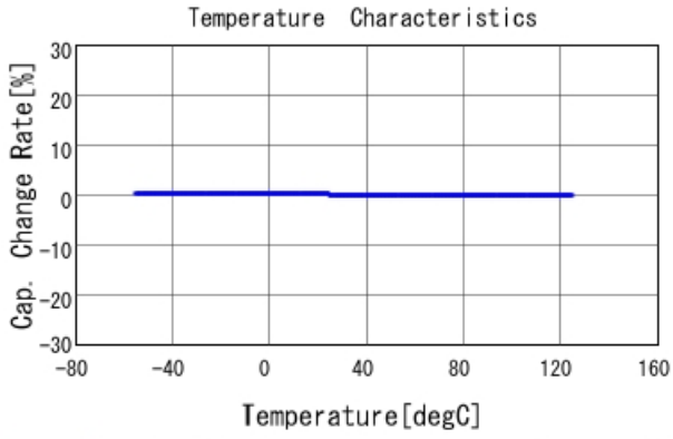
GRM1555C1H820JA01 C-Temp. capchange, DCOV, AC1Vrms
