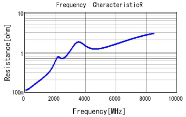
GRM1555C1H820GA01 R DCOV, 25degC
