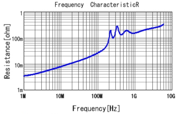
GRM1555C1H682GE01 R DCOV, 25degC
