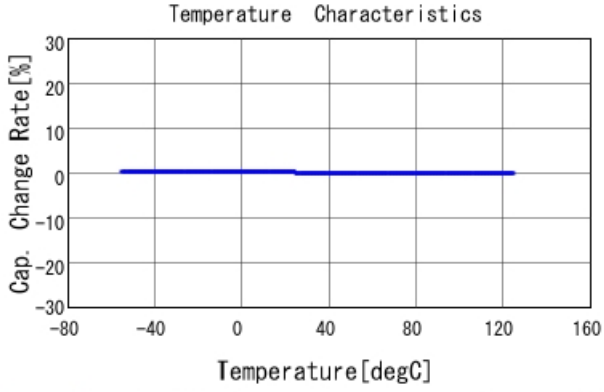
GRM1555C1H682GE01 C-Temp. capchange, DCOV, AC1Vrms
