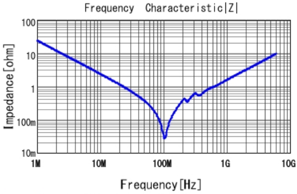
GRM1555C1H682GE01 |Z| DCOV, 25degC
