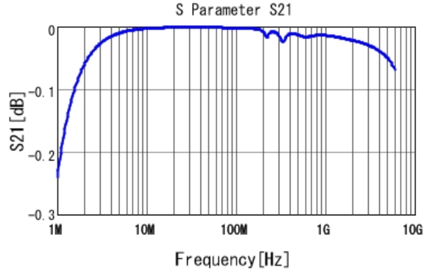
GRM1555C1H682GE01 S21 DCOV, 25degC
