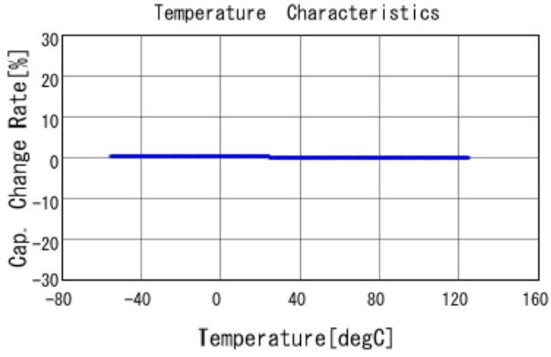
GRM1555C1H681JA01 C-Temp. capchange, DCOV, AC1Vrms
