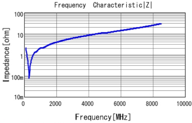
GRM1555C1H681JA01 |Z| DCOV, 25degC
