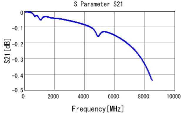
GRM1555C1H681JA01 S21 DCOV, 25degC
