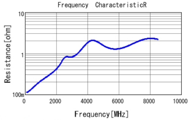
GRM1555C1H680JA01 R DCOV, 25degC
