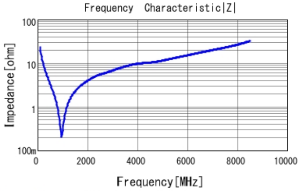
GRM1555C1H680JA01 |Z| DCOV, 25degC
