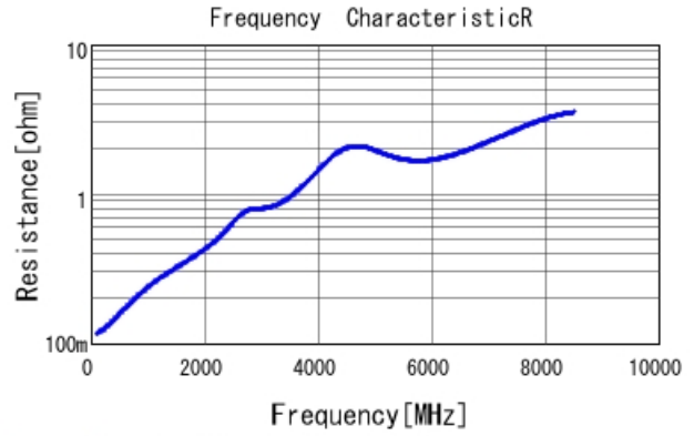
GRM1555C1H620JA01 R DCOV, 25degC
