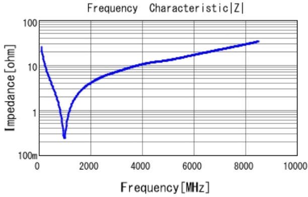
GRM1555C1H620JA01 |Z| DCOV, 25degC
