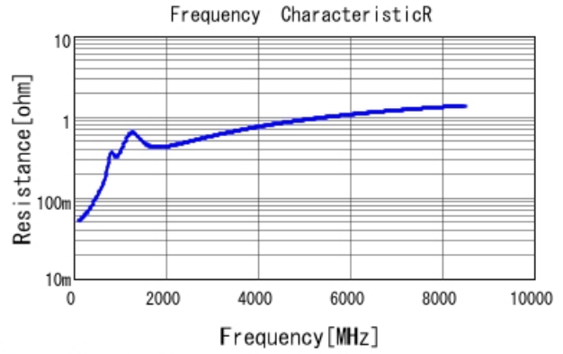
GRM1555C1H561JA01 R DCOV, 25degC
