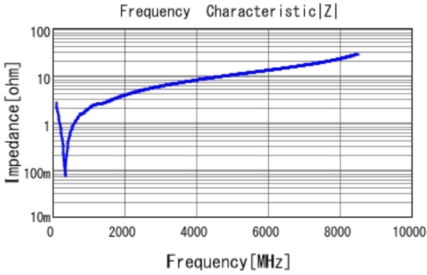
GRM1555C1H561JA01 |Z| DCOV, 25degC
