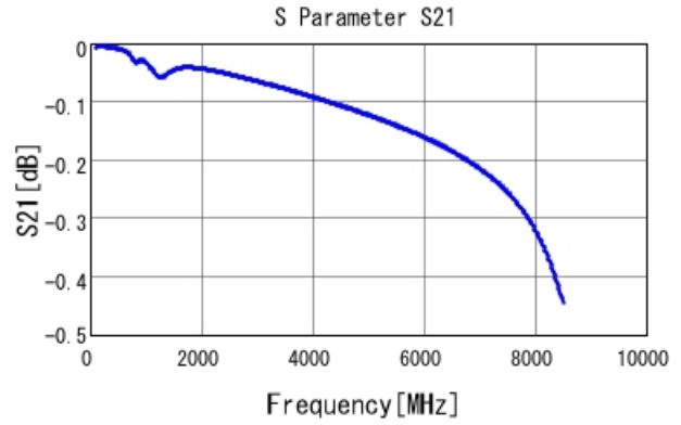
GRM1555C1H561JA01 S21 DCOV, 25degC
