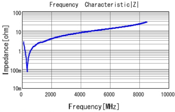
GRM1555C1H561GA01 |Z| DCOV, 25degC
