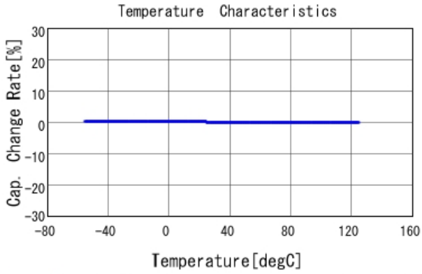
GRM1555C1H560JA01 C-Temp. capchange, DCOV, AC1Vrms
