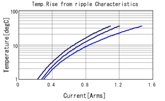
GRM1555C1H560GA01 Temp. rise — 200MHz — 500I
