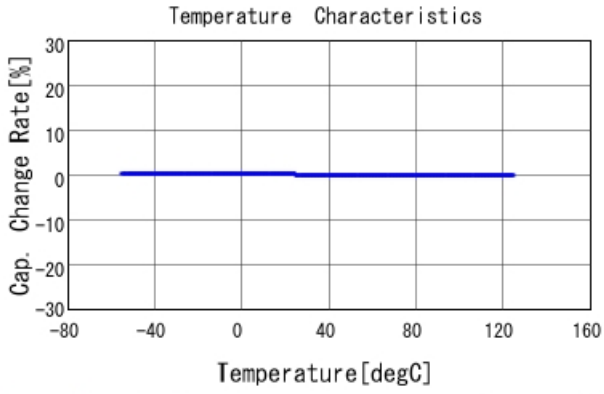
GRM1555C1H560GA01 C-Temp. capchange, DCOV, AC1Vrms
