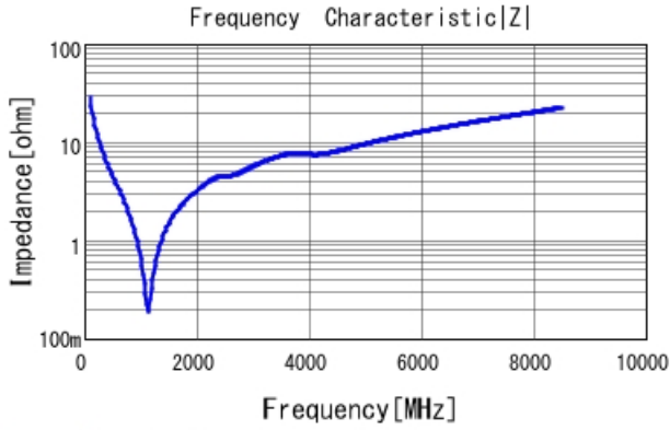
GRM1555C1H560GA01 |Z| DCOV, 25degC
