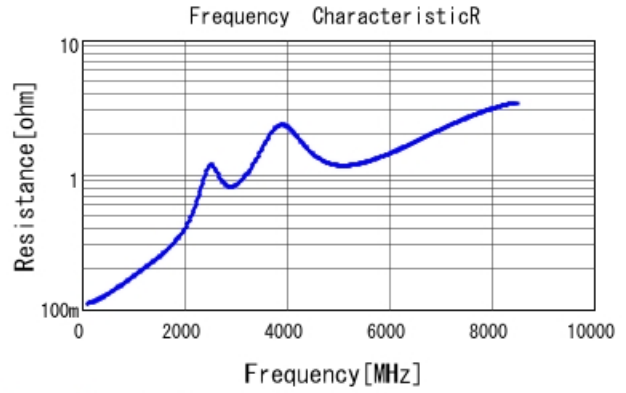
GRM1555C1H560GA01 R DCOV, 25degC
