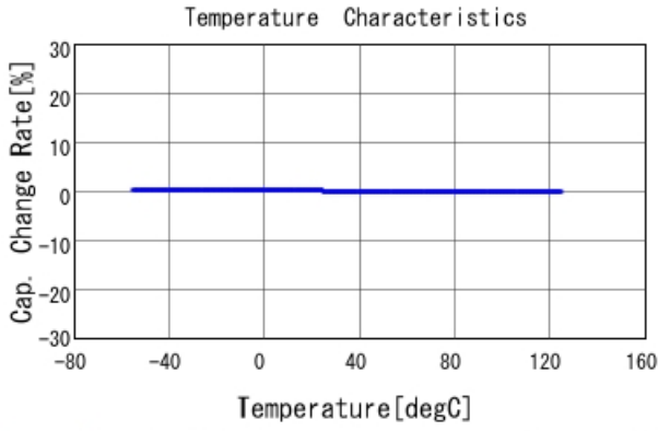
GRM1555C1H510JA01 C-Temp. capchange, DCOV, AC1Vrms
