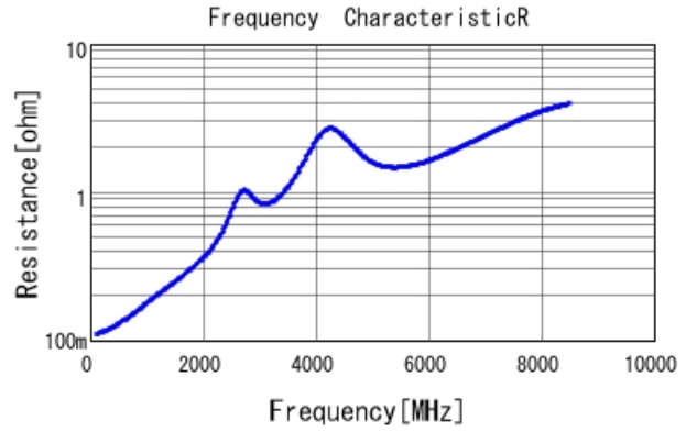
GRM1555C1H510JA01 R DCOV, 25degC
