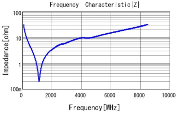
GRM1555C1H510JA01 |Z| DCOV, 25degC
