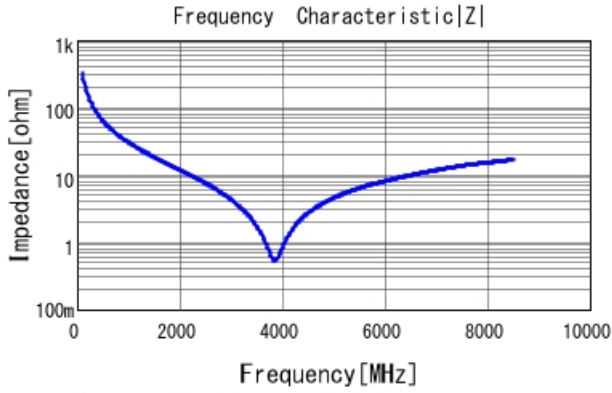
GRM1555C1H4R9CA01 |Z| DCOV, 25degC
