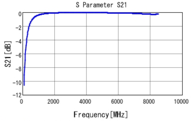
GRM1555C1H4R9CA01 S21 DCOV, 25degC
