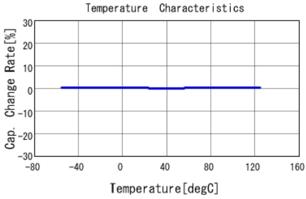
GRM1555C1H4R9CA01 C-Temp. capchange, DCOV, AC1Vrms
