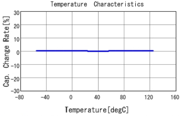
GRM1555C1H4R8CA01 C-Temp. capchange, DCOV, AC1Vrms
