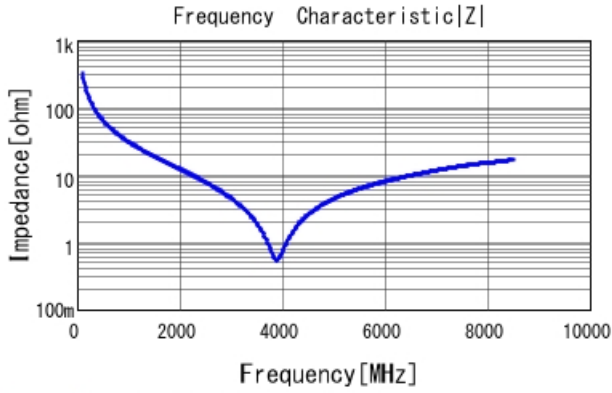
GRM1555C1H4R8CA01 |Z| DCOV, 25degC
