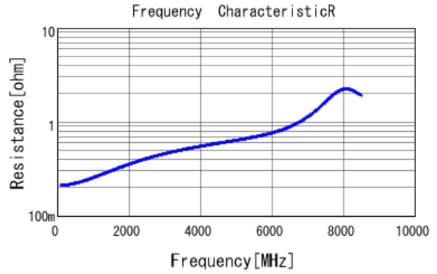
GRM1555C1H4R7BA01 R DCOV, 25degC
