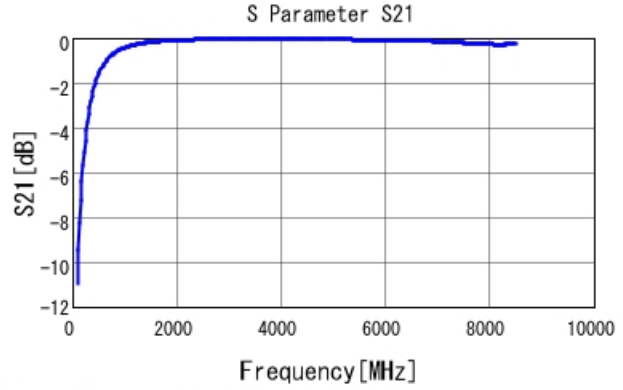
GRM1555C1H4R7BA01 S21 DCOV, 25degC
