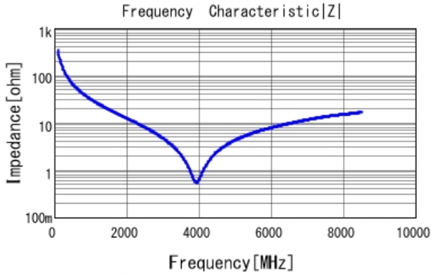
GRM1555C1H4R7BA01 |Z| DCOV, 25degC
