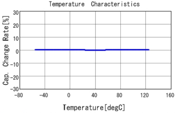
GRM1555C1H4R7BA01 C-Temp. capchange, DCOV, AC1Vrms
