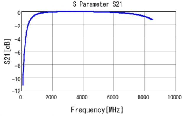
GRM1555C1H4R6WA01 S21 DCOV, 25degC
