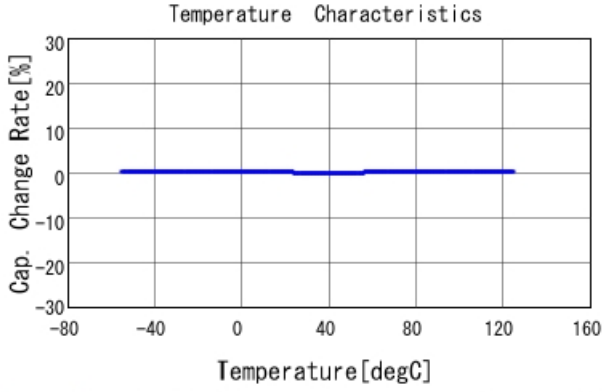
GRM1555C1H4R6WA01 C-Temp. capchange, DCOV, AC1Vrms
