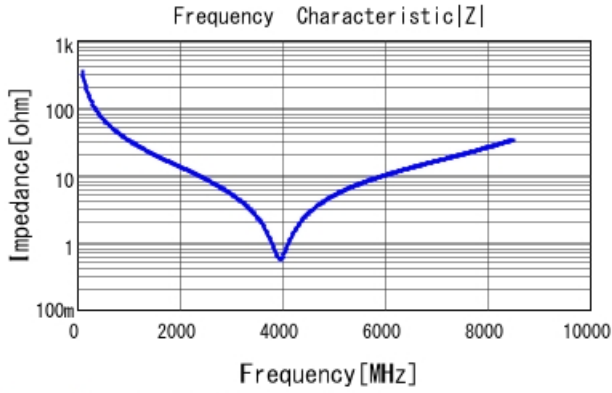
GRM1555C1H4R6WA01 |Z| DCOV, 25degC
