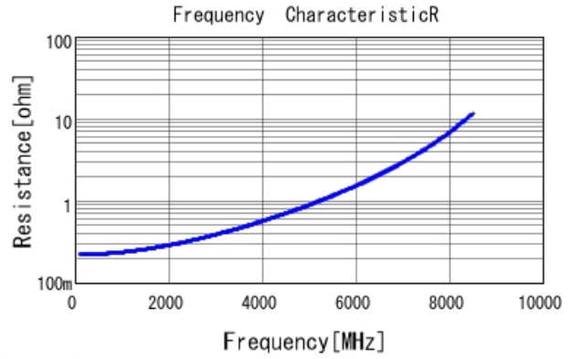
GRM1555C1H4R6WA01 R DCOV, 25degC
