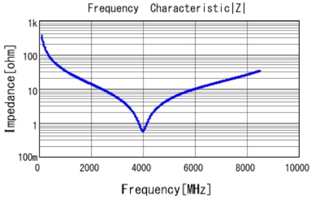
GRM1555C1H4R5WA01 |Z| DCOV, 25degC
