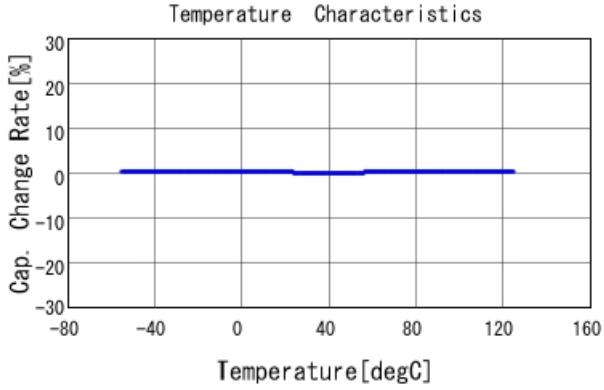
GRM1555C1H4R5WA01 C-Temp. capchange, DC0V, AC1Vrms
