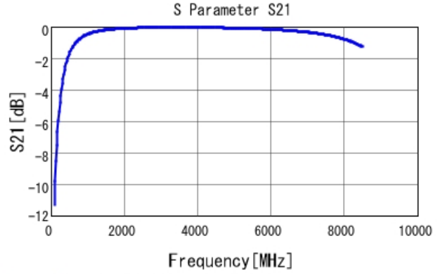
GRM1555C1H4R5WA01 S21 DC0V, 25degC
