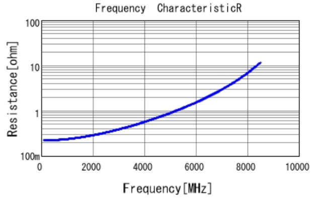
GRM1555C1H4R5WA01 R DCOV, 25degC
