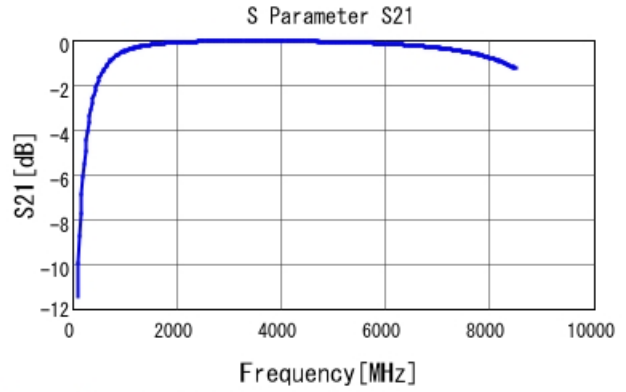
GRM1555C1H4R4WA01 S21 DCOV, 25degC
