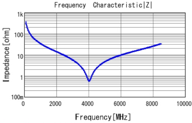
GRM1555C1H4R4WA01 |Z| DCOV, 25degC
