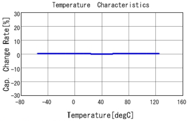
GRM1555C1H4R4WA01 C-Temp. capchange, DCOV, AC1Vrms
