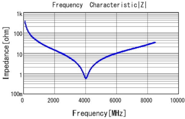
GRM1555C1H4R4CA01 |Z| DCOV, 25degC
