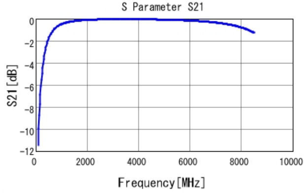
GRM1555C1H4R4CA01 S21 DCOV, 25degC
