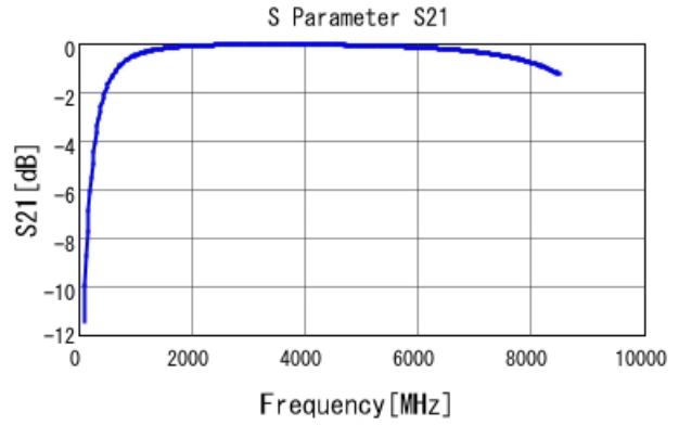
GRM1555C1H4R4BA01 S21 DCOV, 25degC
