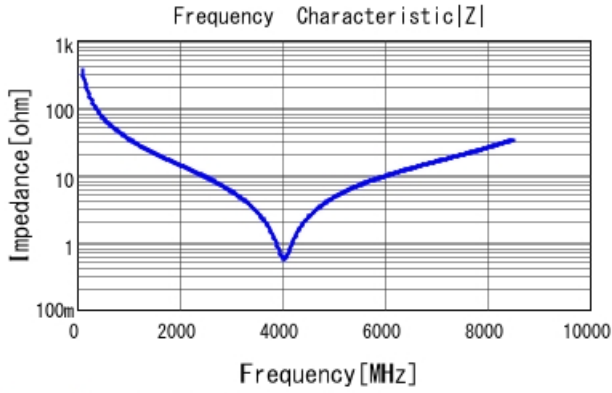
GRM1555C1H4R4BA01 |Z| DCOV, 25degC
