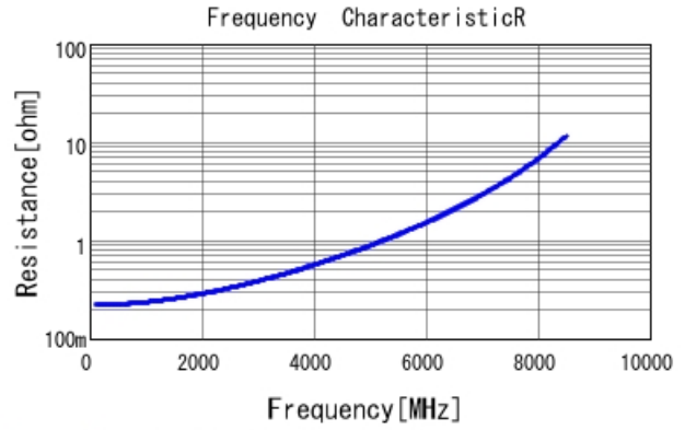
GRM1555C1H4R4BA01 R DCOV, 25degC
