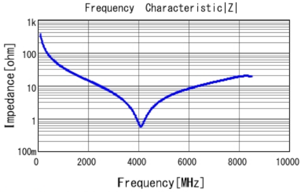
GRM1555C1H4R3CA01 |Z| DCOV, 25degC
