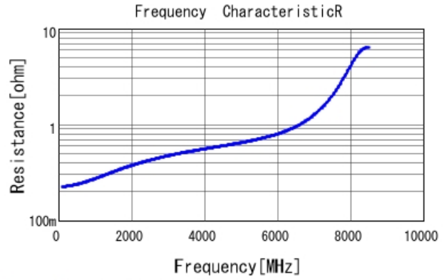
GRM1555C1H4R3CA01 R DCOV, 25degC
