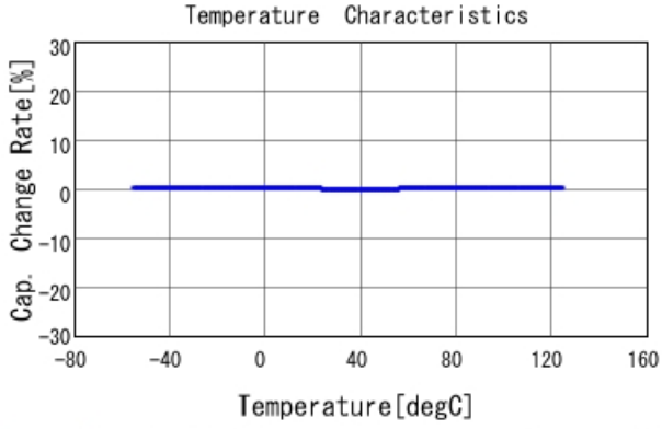
GRM1555C1H4R3CA01 C-Temp. capchange, DCOV, AC1Vrms
