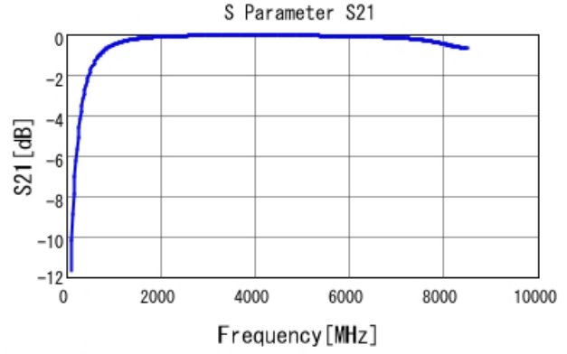
GRM1555C1H4R3CA01 S21 DCOV, 25degC
