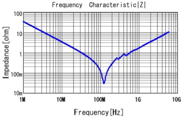
GRM1555C1H472GE01 |Z| DCOV, 25degC
