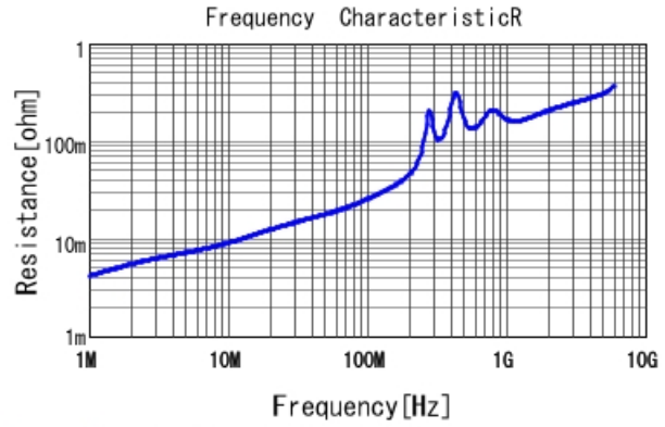
GRM1555C1H472GE01 R DCOV, 25degC
