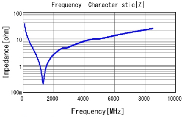
GRM1555C1H430JA01 |Z| DCOV, 25degC
