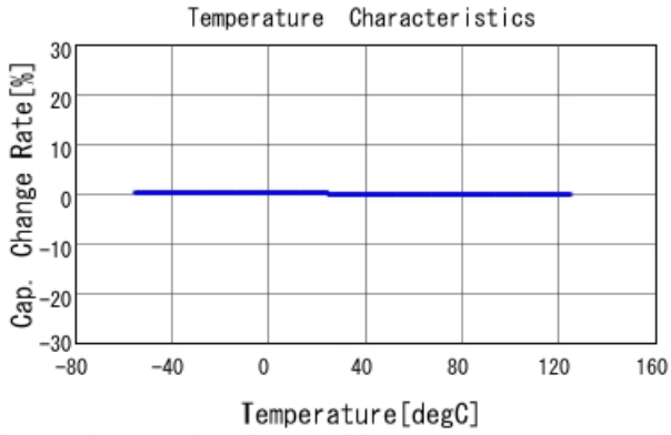
GRM1555C1H430JA01 C-Temp. capchange, DCOV, AC1Vrms
