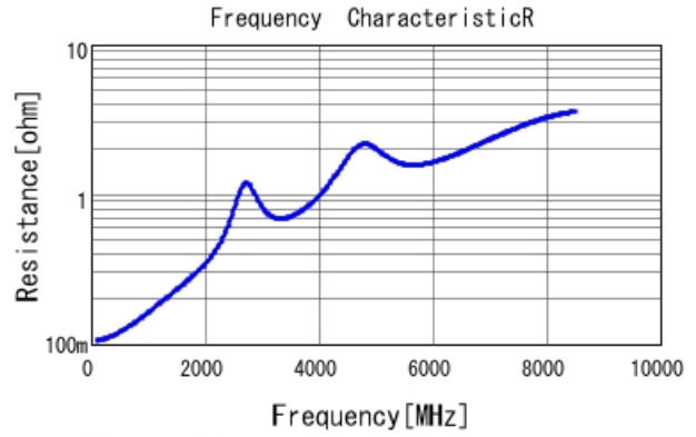
GRM1555C1H430JA01 R DCOV, 25degC
