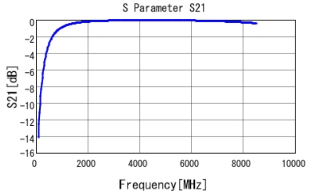
GRM1555C1H3R2BA01 S21 DCOV, 25degC
