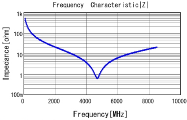
GRM1555C1H3R2BA01 |Z| DCOV, 25degC
