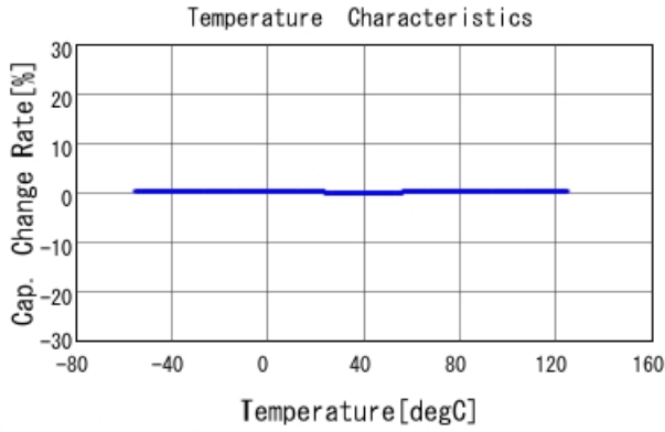
GRM1555C1H3R2BA01 C-Temp. capchange, DCOV, AC1Vrms
