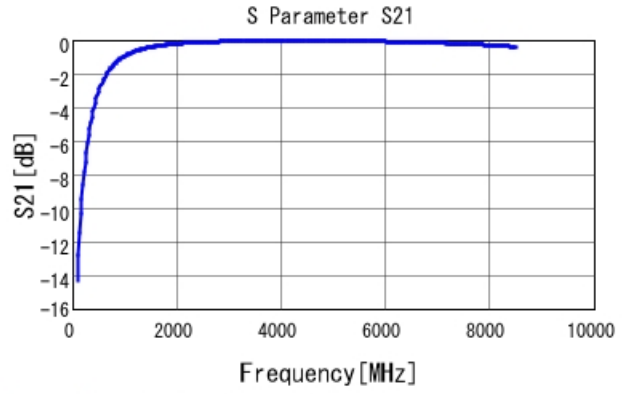
GRM1555C1H3R1WA01 S21 DCOV, 25degC
