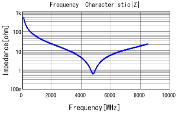
GRM1555C1H3R1WA01 |Z| DCOV, 25degC
