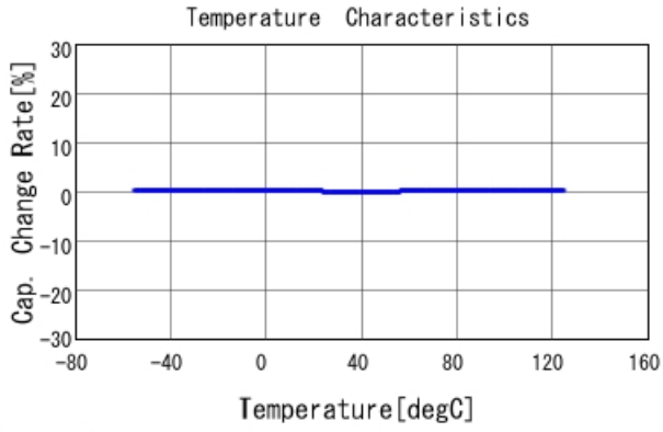
GRM1555C1H3R1WA01 C-Temp. capchange, DCOV, AC1Vrms
