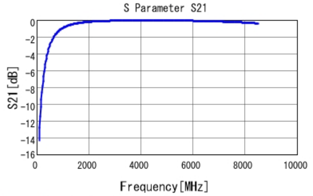
GRM1555C1H3R1CA01 S21 DCOV, 25degC
