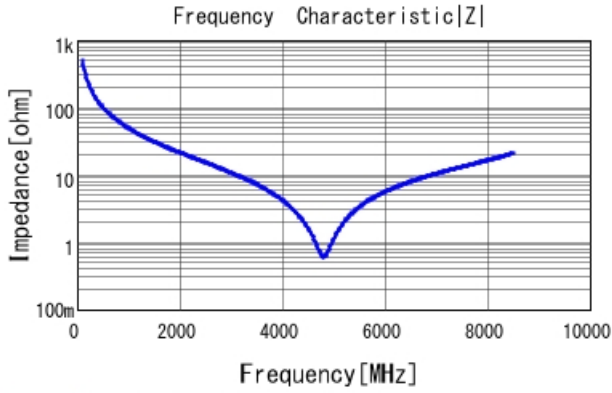
GRM1555C1H3R1CA01 |Z| DCOV, 25degC
