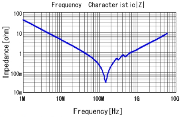
GRM1555C1H392GE01 |Z| DCOV, 25degC
