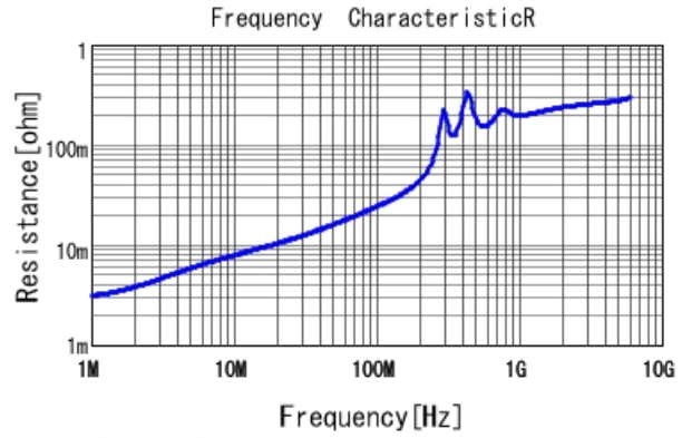
GRM1555C1H392GE01 R DCOV, 25degC
