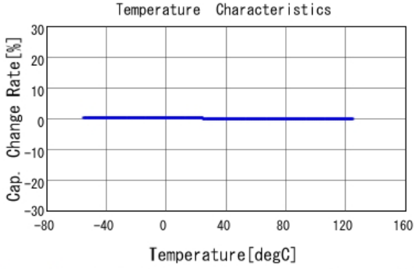
GRM1555C1H391JA01 C-Temp. capchange, DCOV, AC1Vrms
