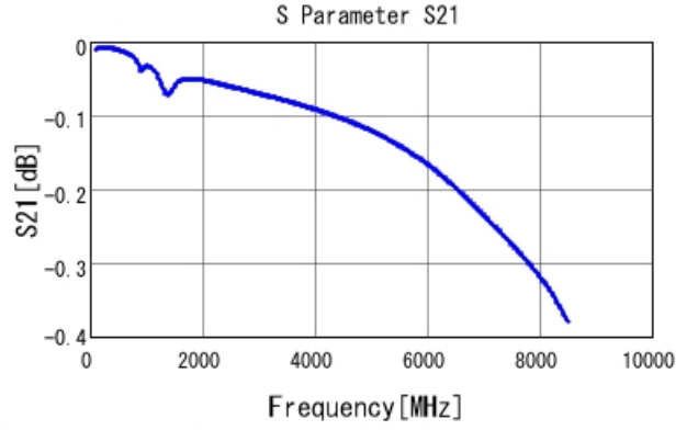
GRM1555C1H391JA01 S21 DCOV, 25degC
