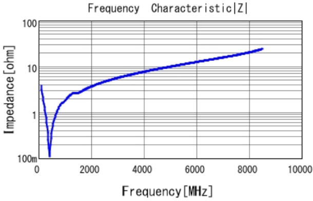
GRM1555C1H391JA01 |Z| DCOV, 25degC
