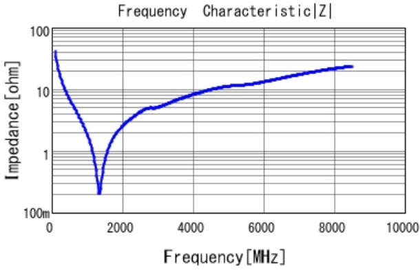
GRM1555C1H390JA01 |Z| DCOV, 25degC
