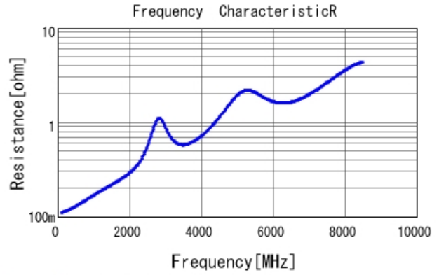
GRM1555C1H390JA01 R DCOV, 25degC
