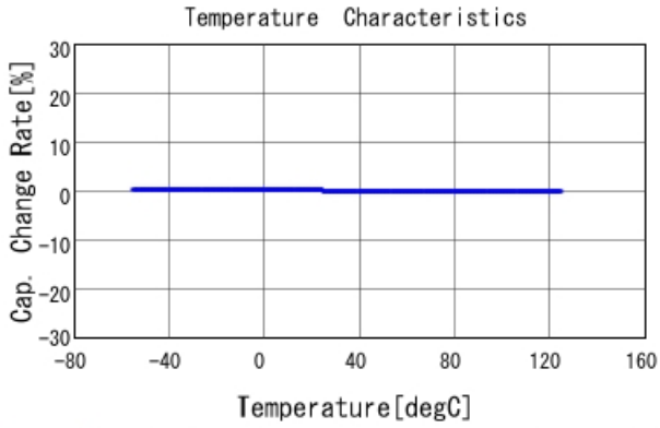
GRM1555C1H330JA01 C-Temp. capchange, DCOV, AC1Vrms
