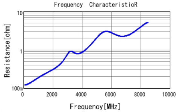
GRM1555C1H330JA01 R DCOV, 25degC
