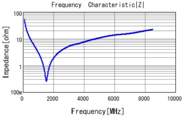
GRM1555C1H300JA01 |Z| DCOV, 25degC
