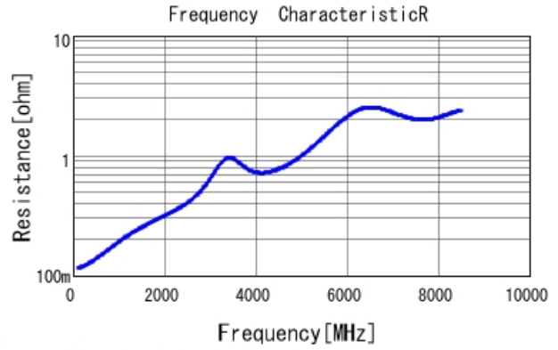
GRM1555C1H300JA01 R DCOV, 25degC
