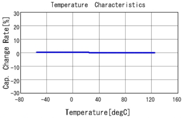
GRM1555C1H300JA01 C-Temp. capchange, DCOV, AC1Vrms
