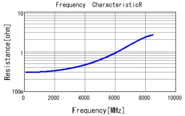
GRM1555C1H2R6BA01 R DCOV, 25degC
