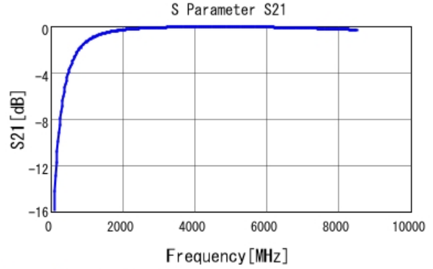
GRM1555C1H2R6BA01 S21 DCOV, 25degC
