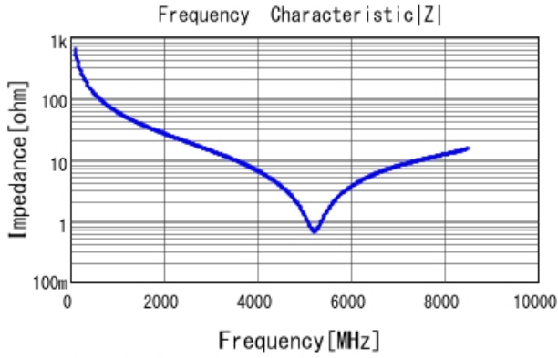
GRM1555C1H2R6BA01 |Z| DCOV, 25degC
