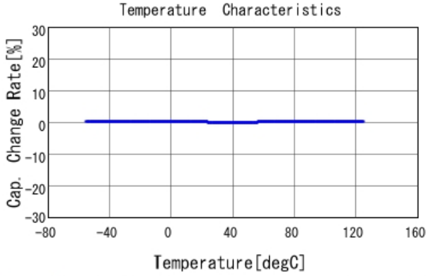
GRM1555C1H2R6BA01 C-Temp. capchange, DCOV, AC1Vrms
