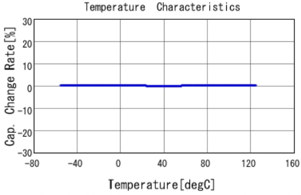
GRM1555C1H2R3CA01 C-Temp. capchange, DCOV, AC1Vrms
