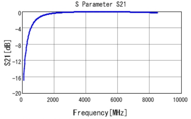
GRM1555C1H2R3CA01 S21 DCOV, 25degC
