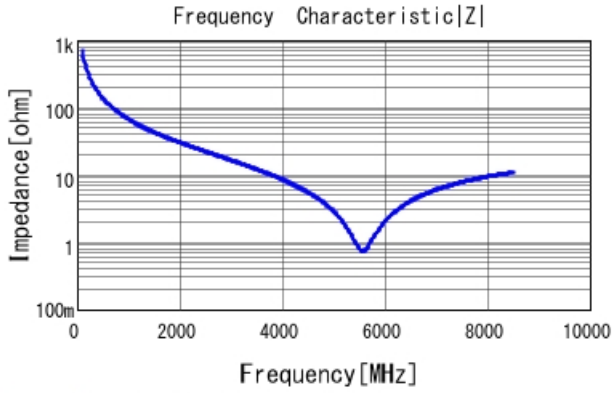
GRM1555C1H2R3CA01 |Z| DCOV, 25degC
