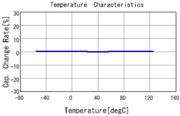
GRM1555C1H2R0BA01 C-Temp. capchange, DCOV, AC1Vrms
