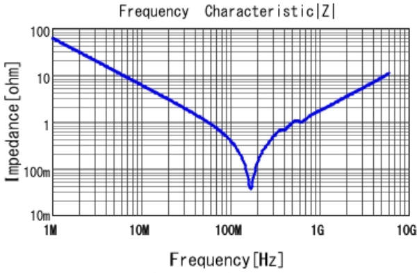
GRM1555C1H272JE01 |Z| DCOV, 25degC
