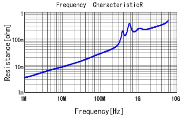
GRM1555C1H272JE01 R DCOV, 25degC
