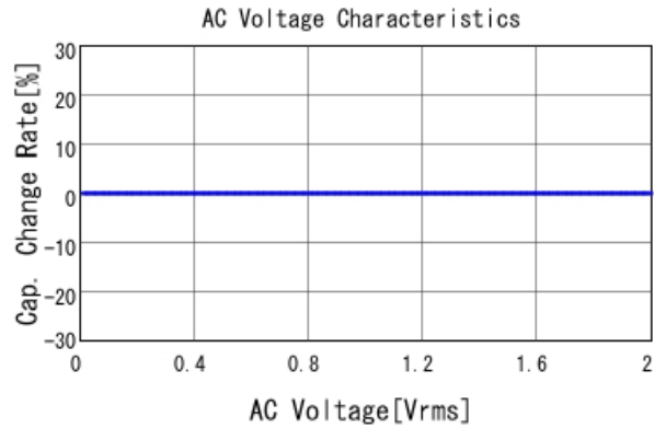
GRM1555C1H272JE01 C-AC Voltage capchange, DCOV, 25
