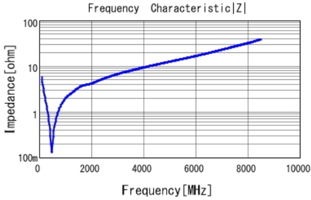
GRM1555C1H271JA01 |Z| DCOV, 25degC
