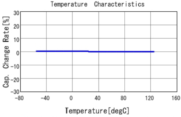
GRM1555C1H270GA01 C-Temp. capchange, DCOV, AC1Vrms
