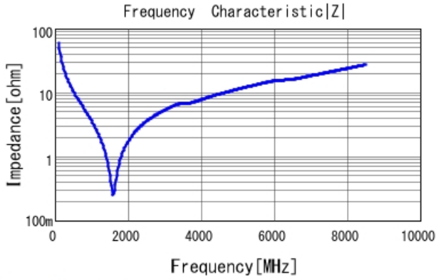
GRM1555C1H270GA01 |Z| DCOV, 25degC
