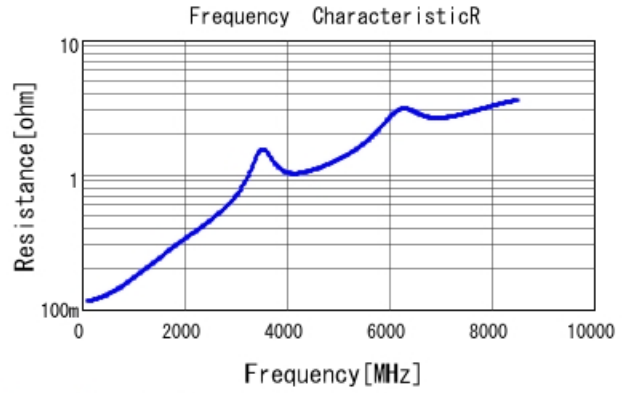
GRM1555C1H270GA01 R DCOV, 25degC
