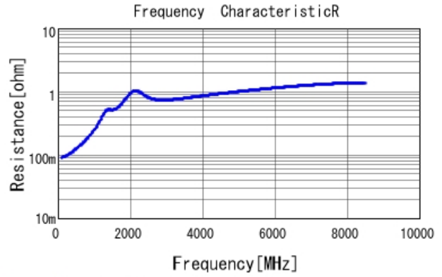
GRM1555C1H221JA01 R DCOV, 25degC
