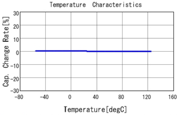
GRM1555C1H221GA01 C-Temp. capchange, DCOV, AC1Vrms
