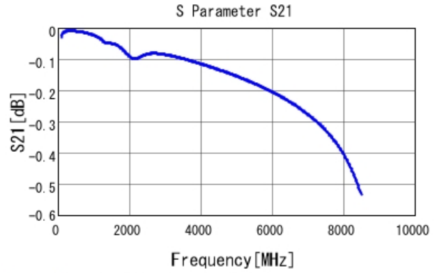
GRM1555C1H221GA01 S21 DCOV, 25degC
