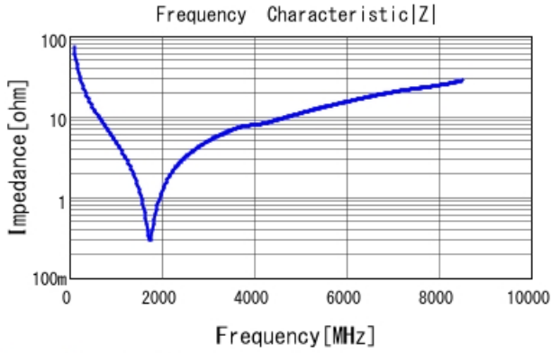
GRM1555C1H220JA01 |Z| DCOV, 25degC
