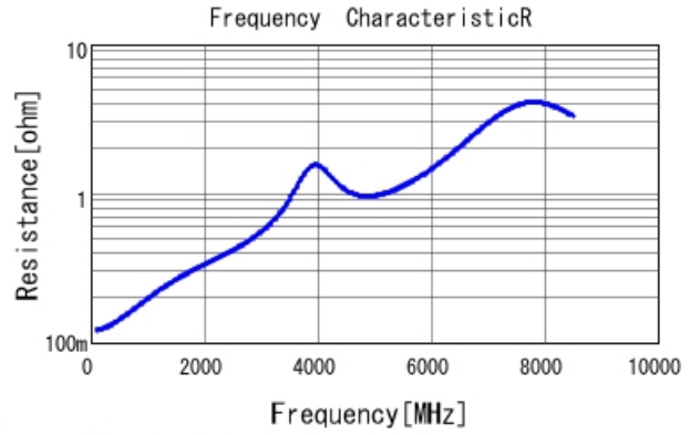
GRM1555C1H220JA01 R DCOV, 25degC
