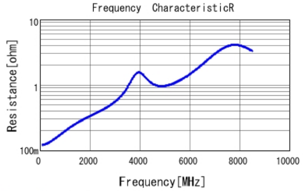
GRM1555C1H220GA01 R DCOV, 25degC
