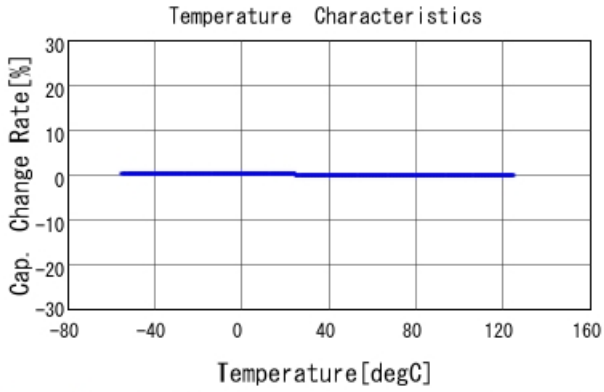
GRM1555C1H220GA01 C-Temp. capchange, DCOV, AC1Vrms
