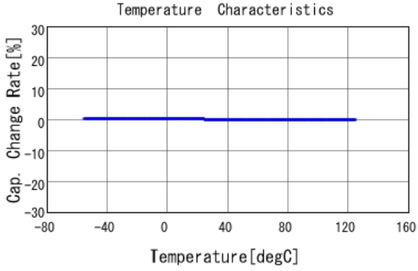
GRM1555C1H200JA01 C-Temp. capchange, DCOV, AC1Vrms
