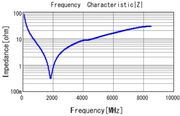
GRM1555C1H200JA01 |Z| DCOV, 25degC
