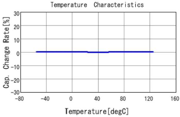
GRM1555C1H1R6BA01 C-Temp. capchange, DCOV, AC1Vrms
