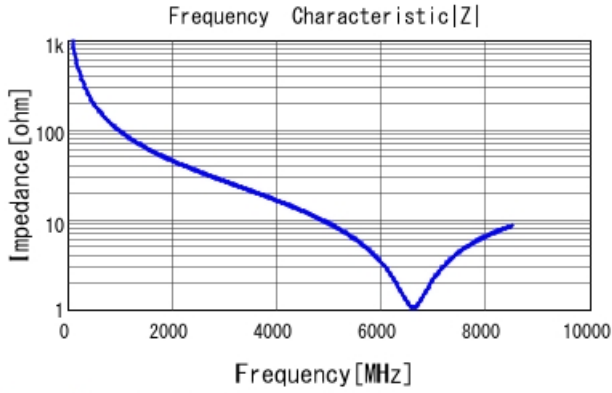
GRM1555C1H1R6BA01 |Z| DCOV, 25degC
