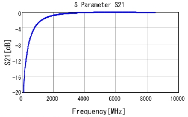
GRM1555C1H1R6BA01 S21 DCOV, 25degC
